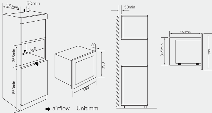
Dimension chart
